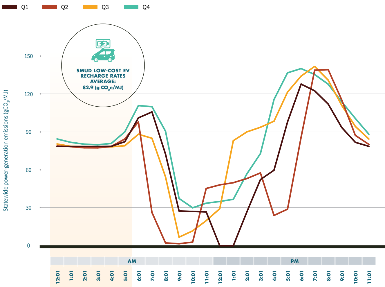
FIGURE 12. CALIFORNIA POWER PLANT GHG EMISSIONS
