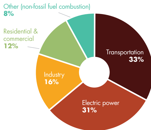
FIGURE 17. U.S. ANTHROPOGENIC CO 2 EMISSIONS BY SOURCE (1990-2020)
