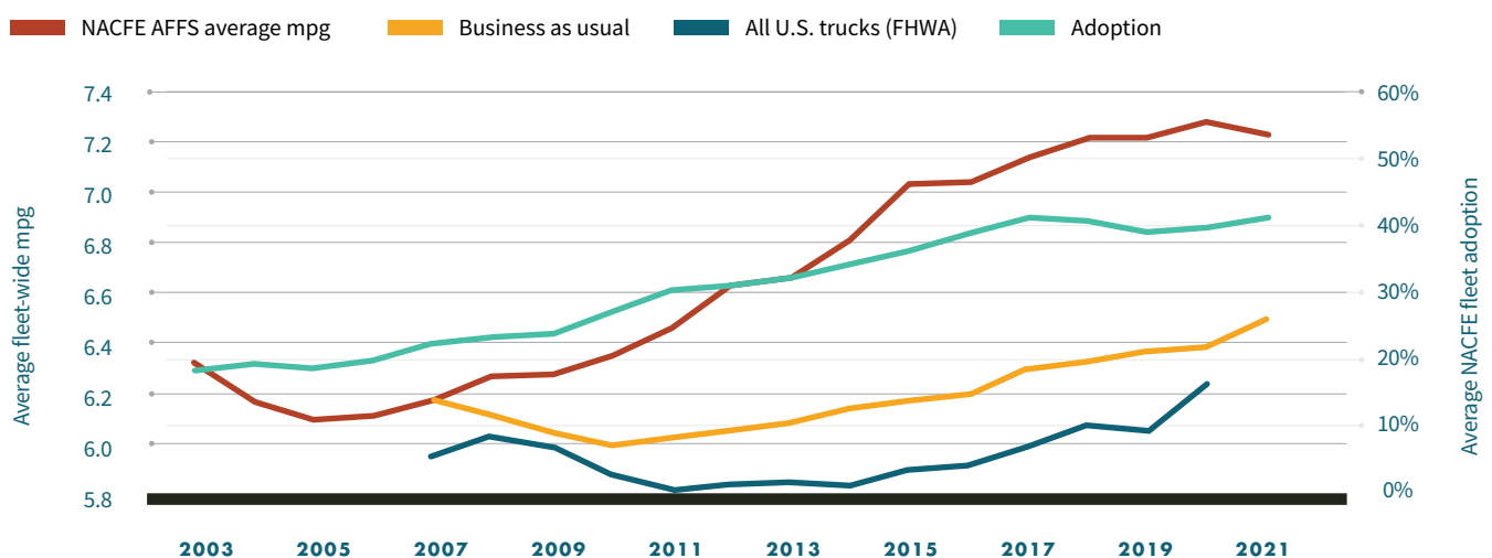
FIGURE 73. AVERAGE FLEET-WIDE FUEL ECONOMY OVER TIME
