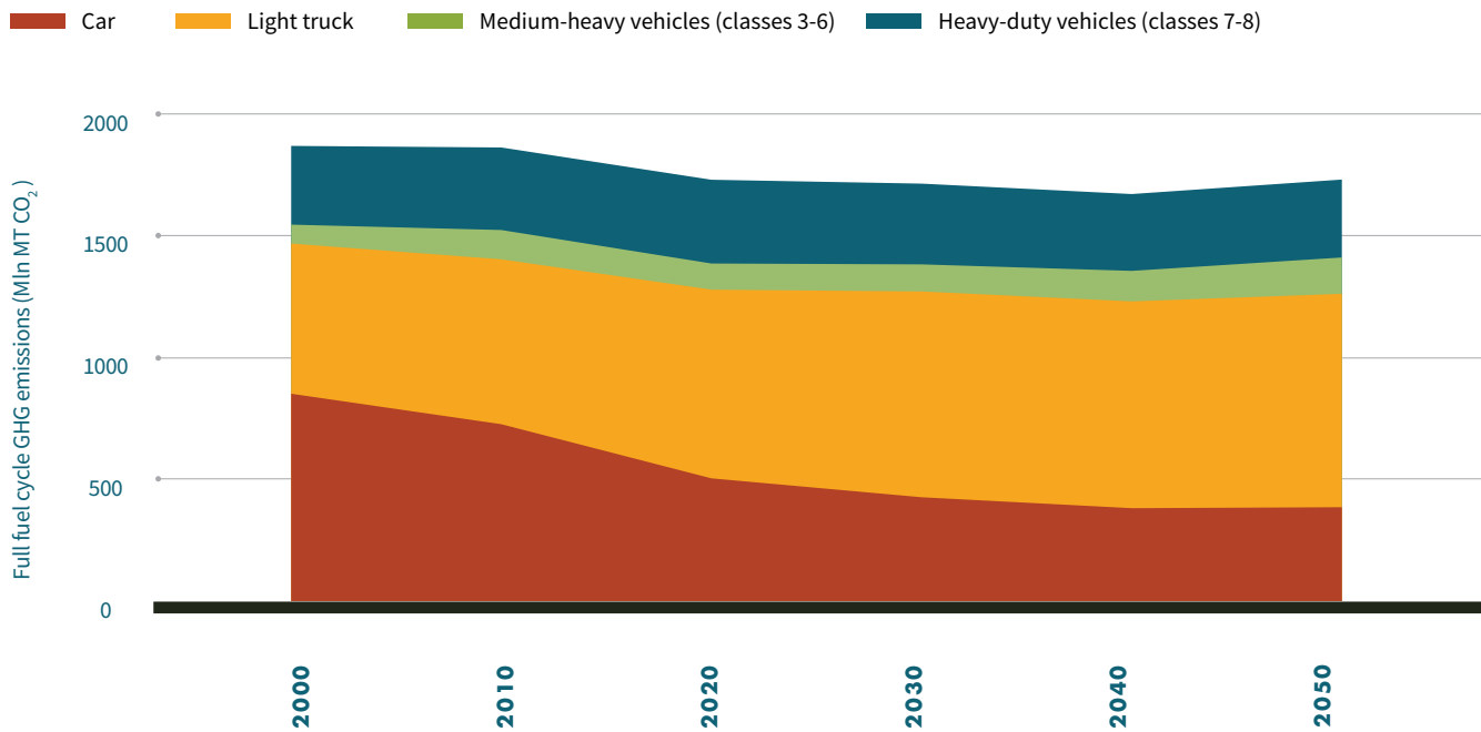
FIGURE 11. ON-ROAD VEHICLES GHG EMISSIONS
