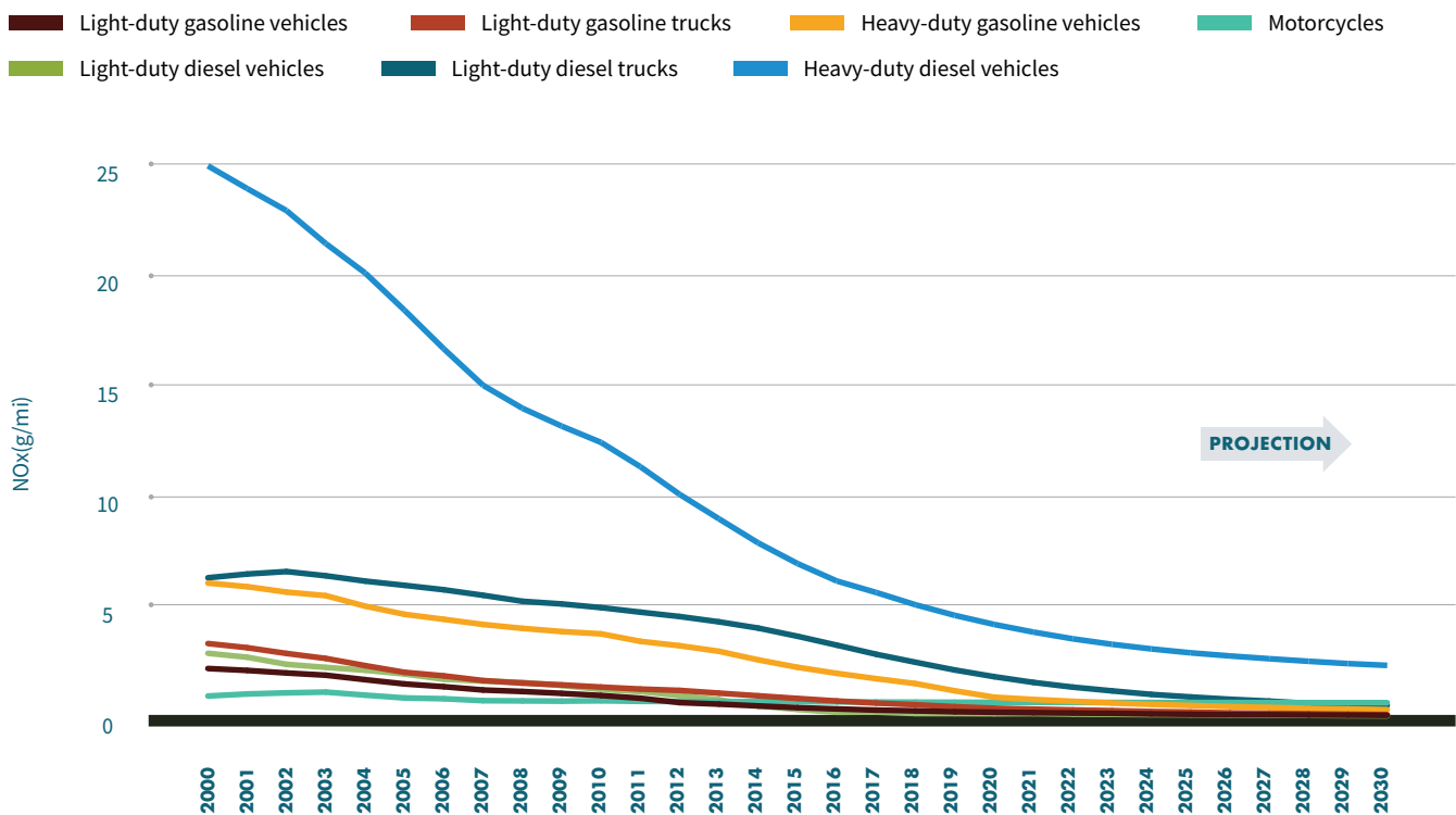
FIGURE 15. ESTIMATED NATIONAL AVERAGE NO x EMISSIONS RATES PER VEHICLE USING GASOLINE AND DIESEL
